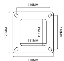
FOOT PLATE
